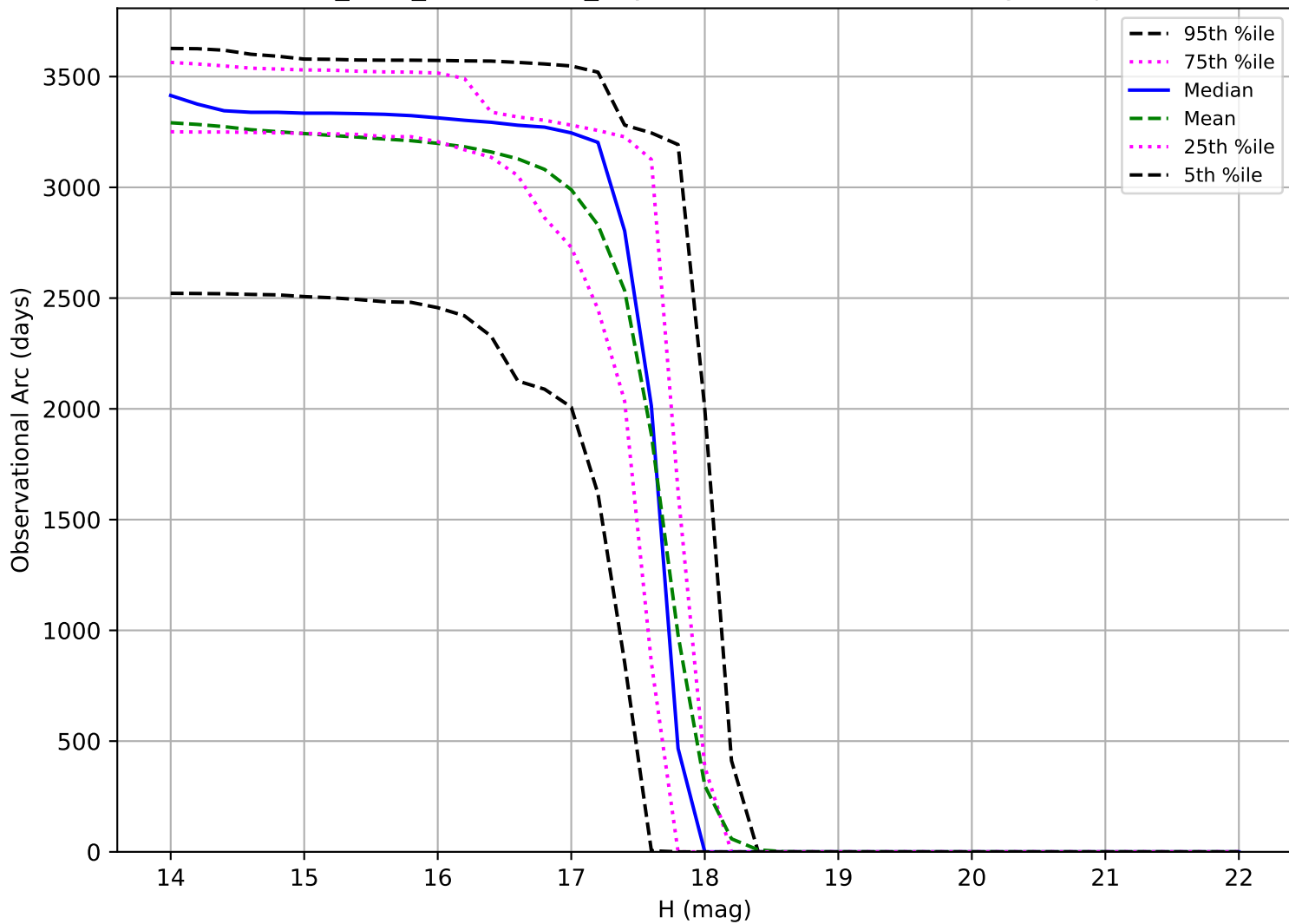
start_date_do-360v3.4_10yrs: Observational Arc Length Trojan
