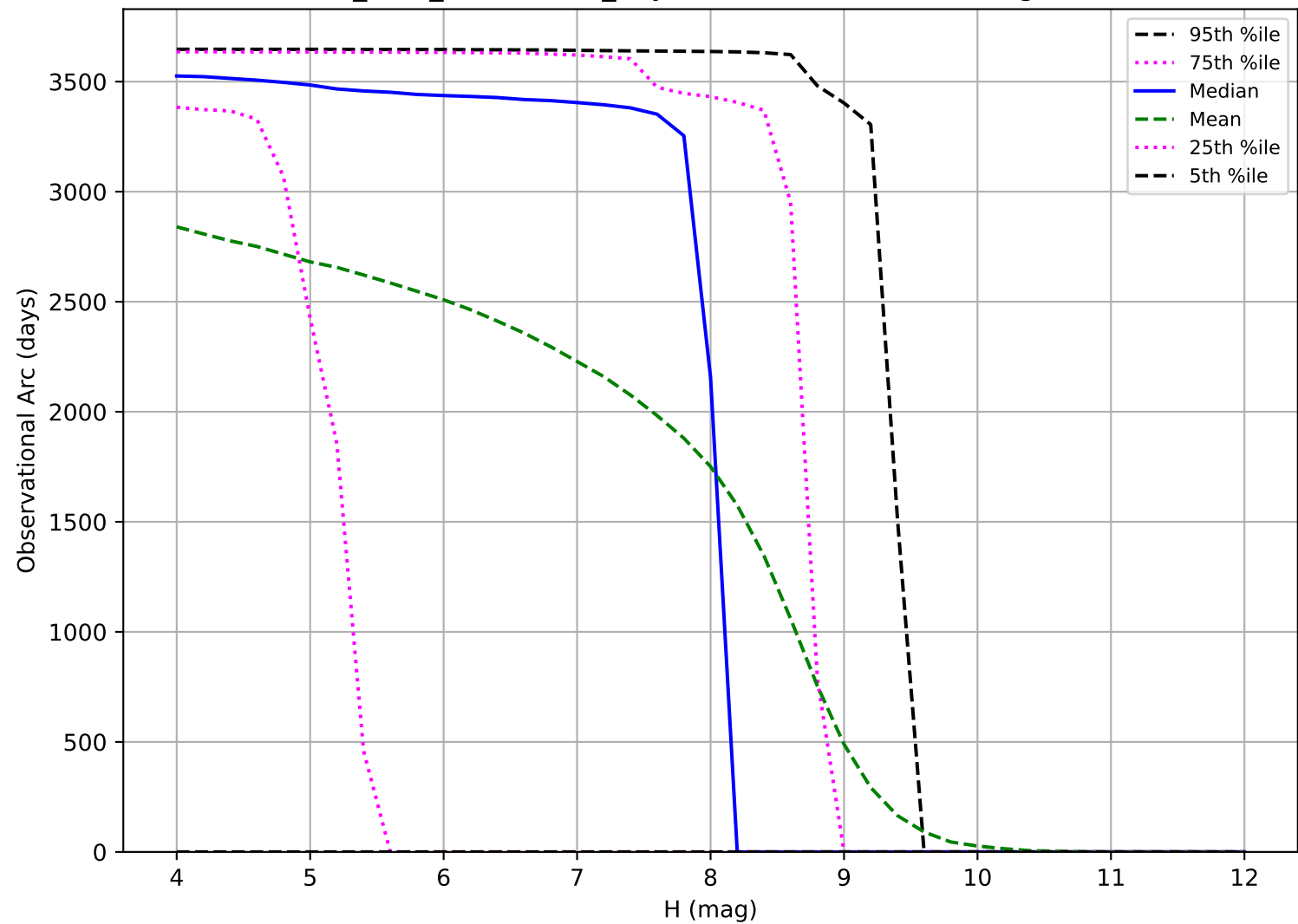
start_date_do-360v3.4_10yrs: Observational Arc Length TNO
