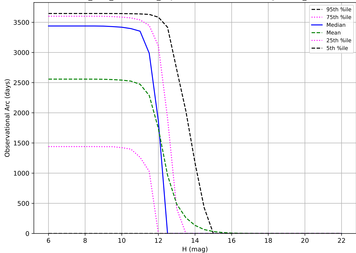
start_date_do-360v3.4_10yrs: Observational Arc Length OCC_r20
