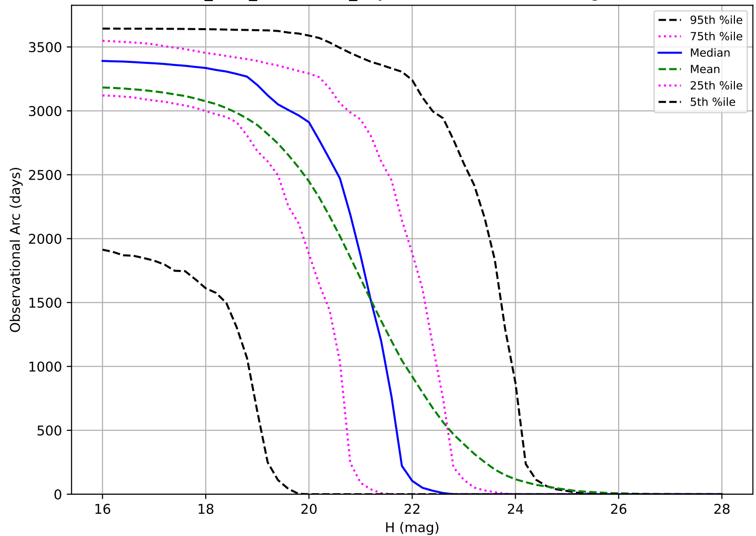
start_date_do-360v3.4_10yrs: Observational Arc Length NEO
