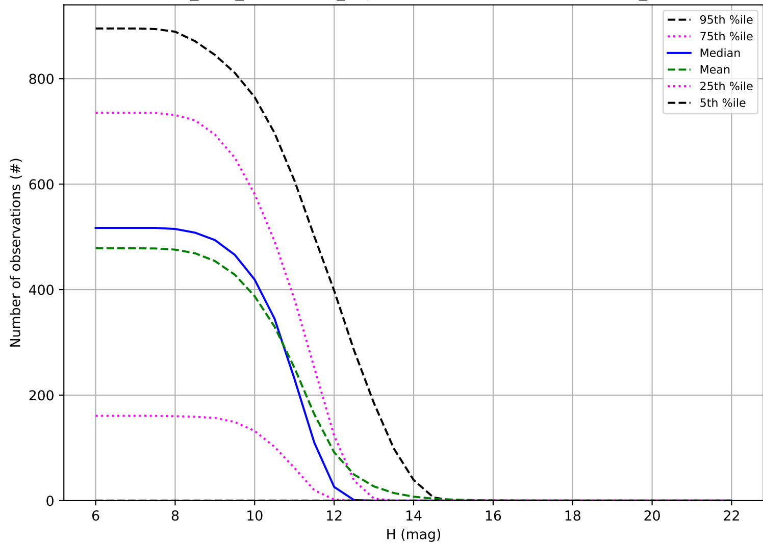
start_date_do-360v3.4_10yrs: Number of observations OCC_r20
