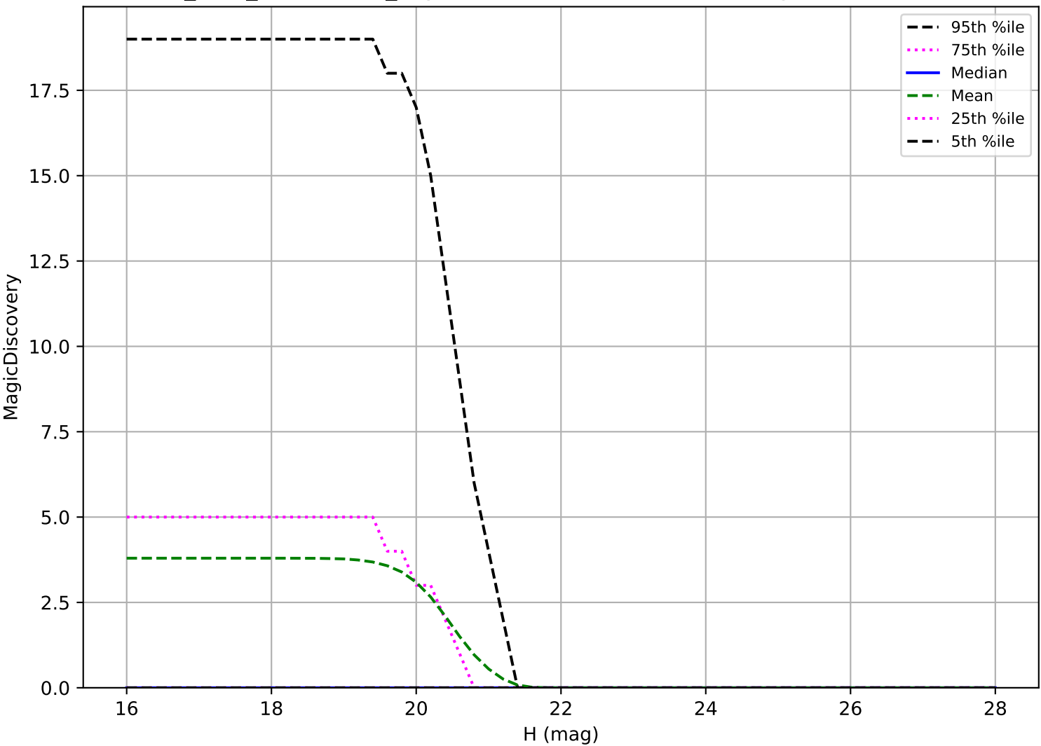
start_date_do-360v3.4_10yrs: Vatira 6 detections in 60 nights detection loss
