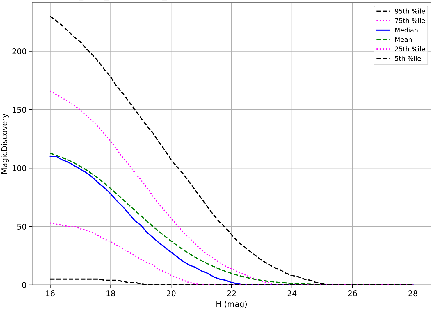
start_date_do-360v3.4_10yrs: NEO 6 detections in 60 nights detection loss
