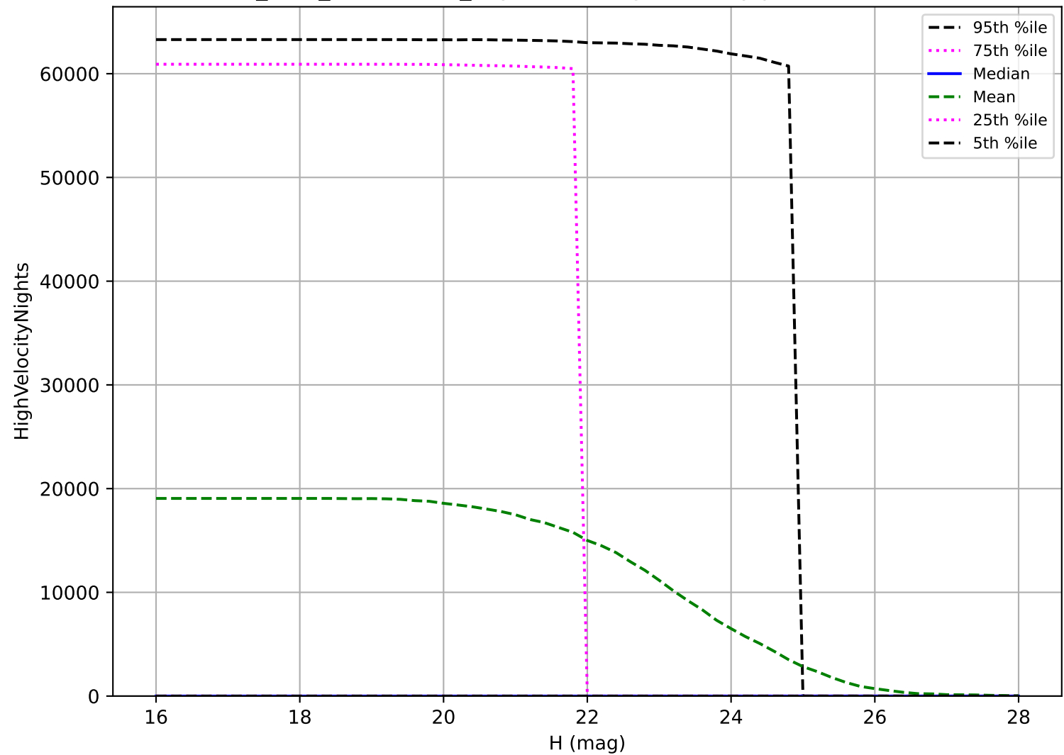
start_date_do-360v3.4_10yrs: NEO High velocity pair detection loss
