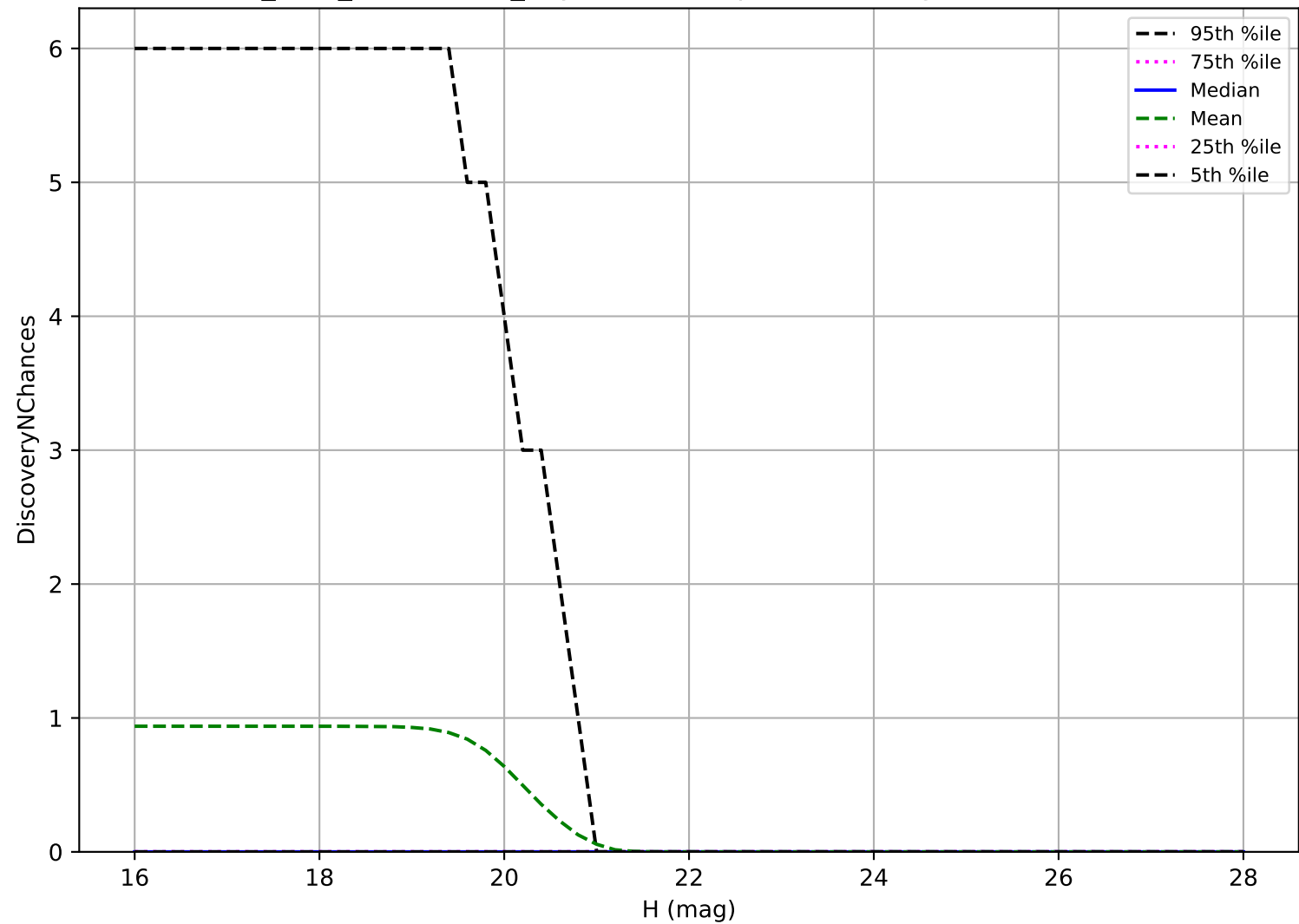
start_date_do-360v3.4_10yrs: Vatira 3 pairs in 15 nights detection loss
