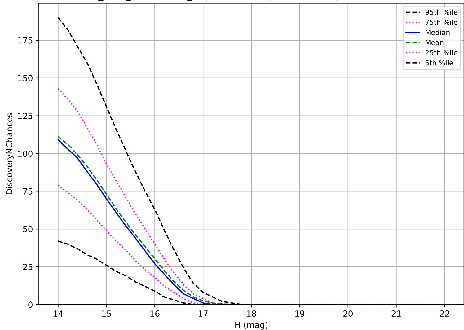
start_date_do-360v3.4_10yrs: Trojan 3 pairs in 15 nights detection loss
