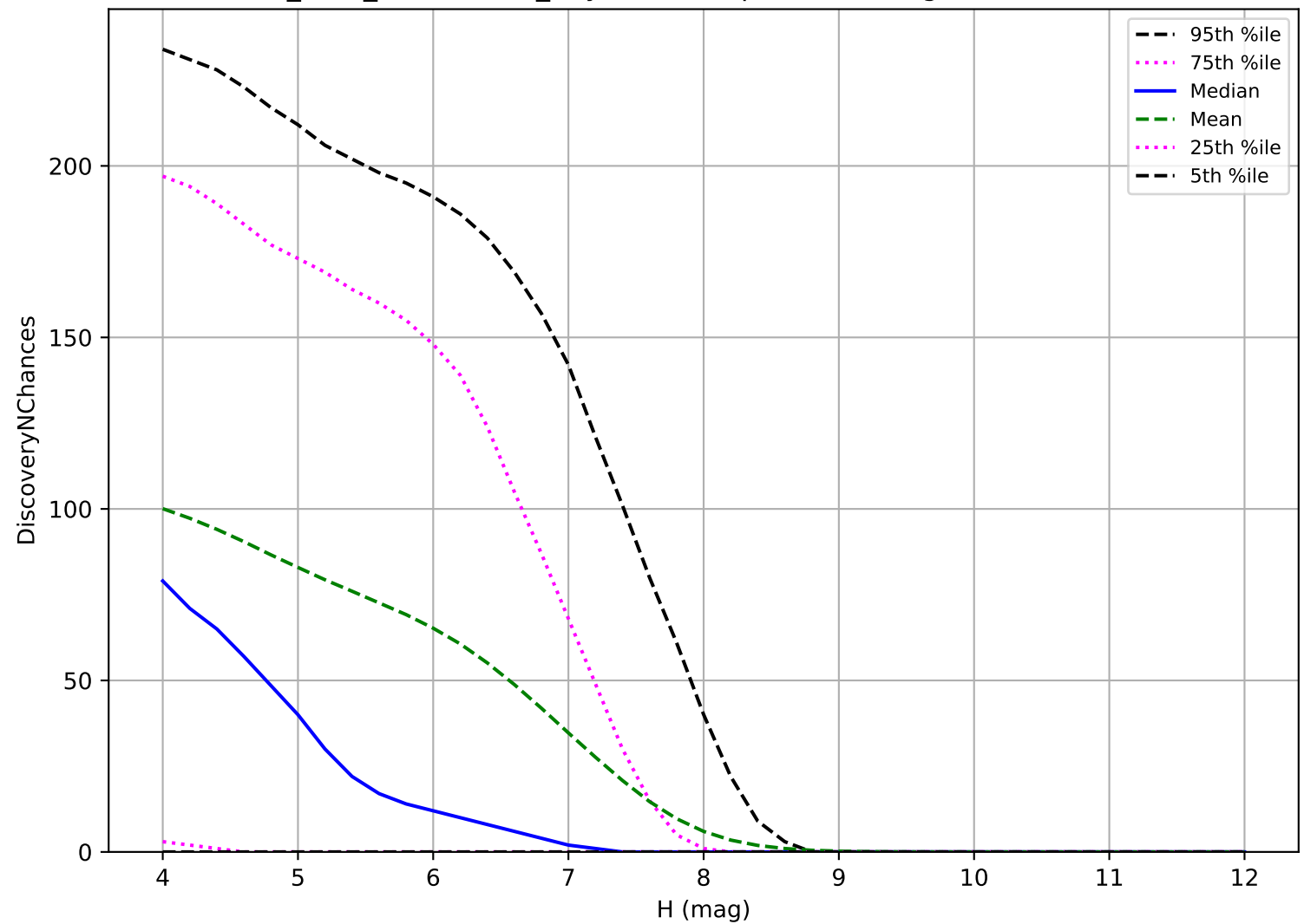
start_date_do-360v3.4_10yrs: TNO 3 pairs in 15 nights detection loss
