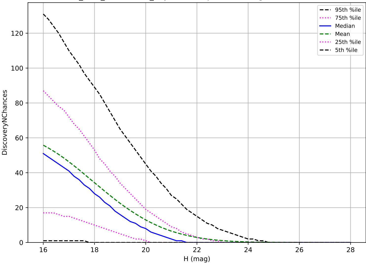
start_date_do-360v3.4_10yrs: PHA 3 pairs in 15 nights detection loss
