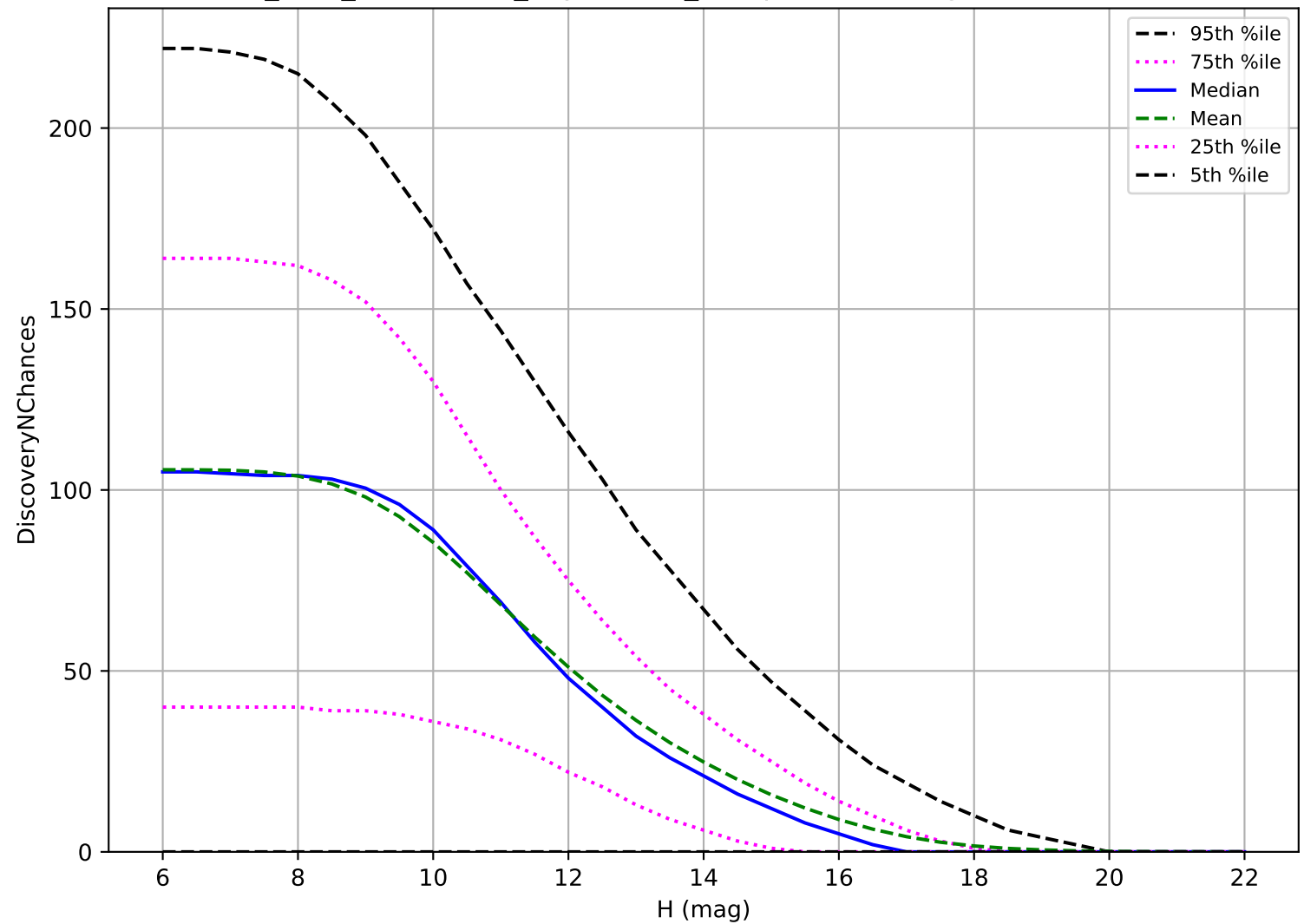
start_date_do-360v3.4_10yrs: OCC_r5 3 pairs in 15 nights detection loss
