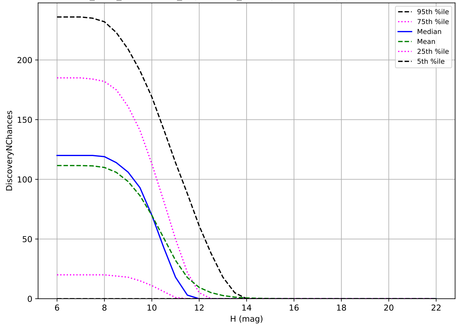
start_date_do-360v3.4_10yrs: OCC_r20 3 pairs in 15 nights detection loss
