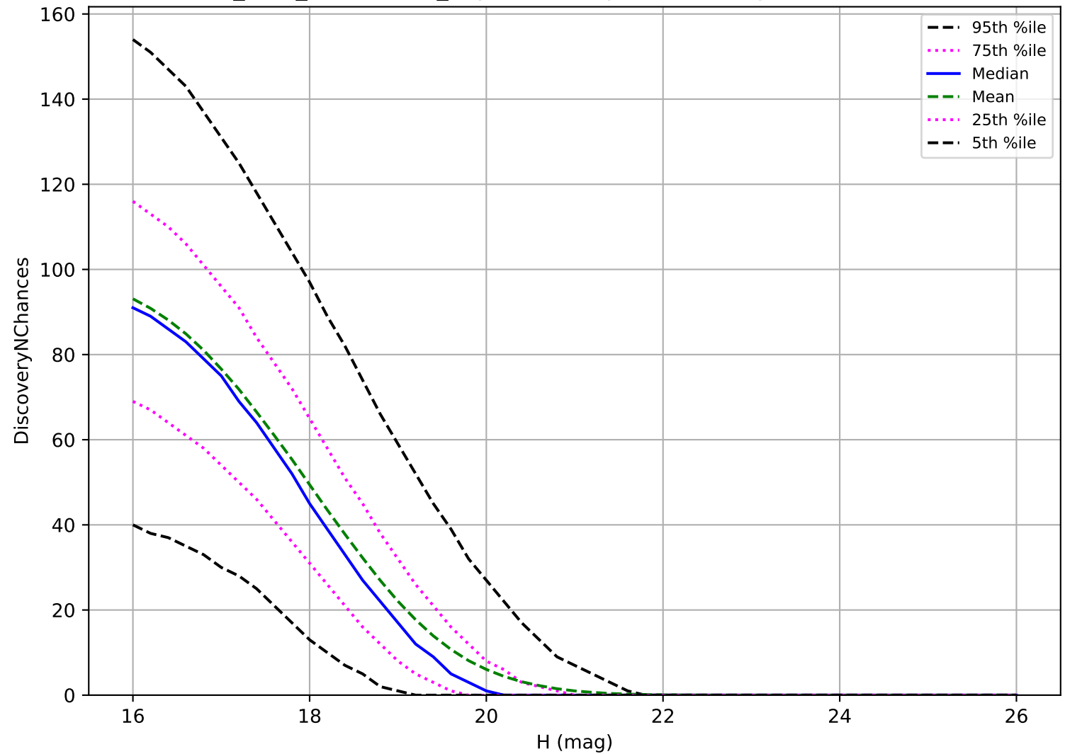
start_date_do-360v3.4_10yrs: MBA 3 pairs in 15 nights detection loss
