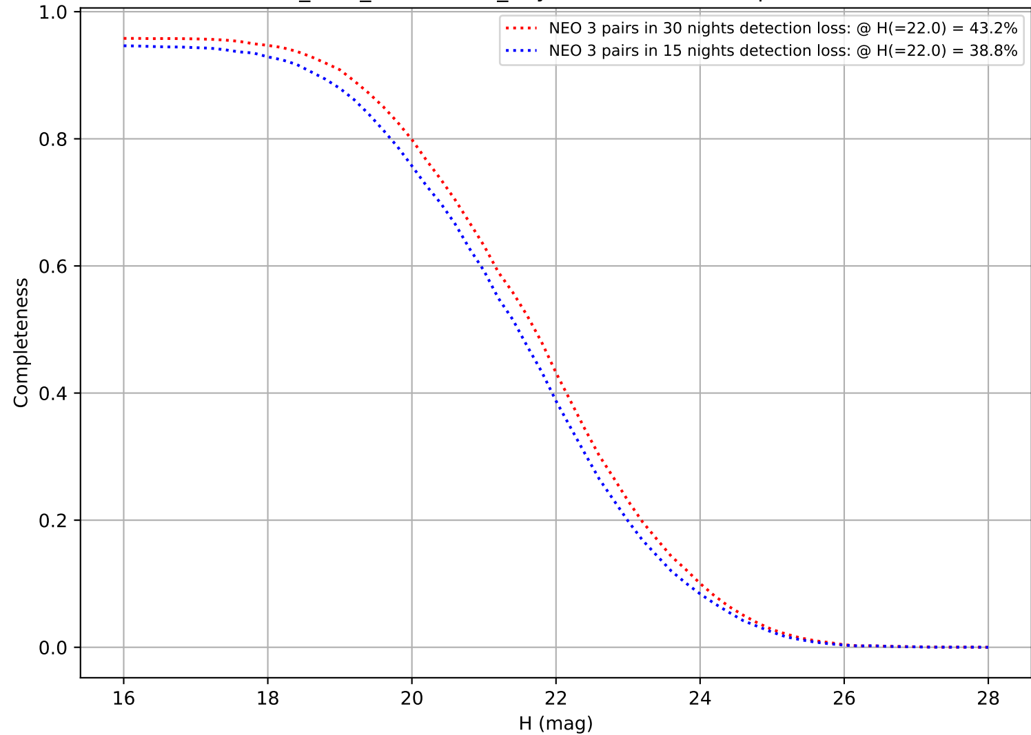
start_date_do-360v3.4_10yrs: DifferentialCompleteness
