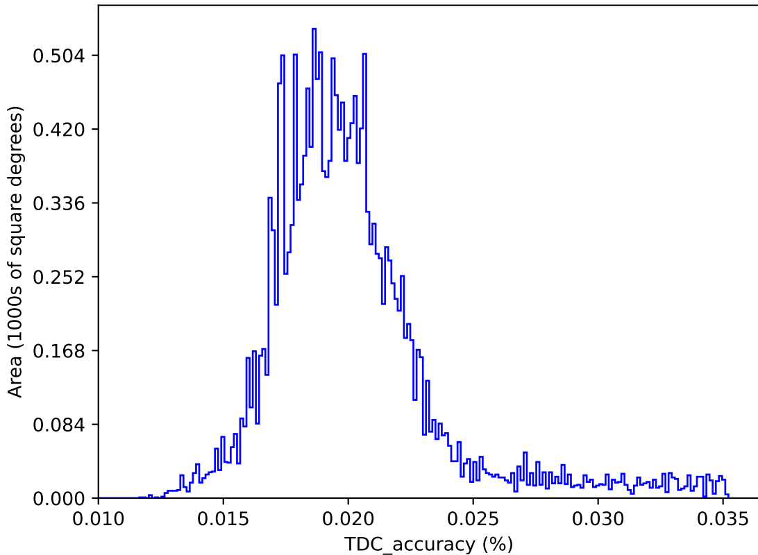
start_date_do-360v3.4_10yrs : TDC_accuracy
