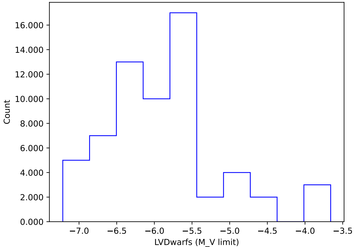
start_date_do-360v3.4_10yrs gi: LVDwarfs
