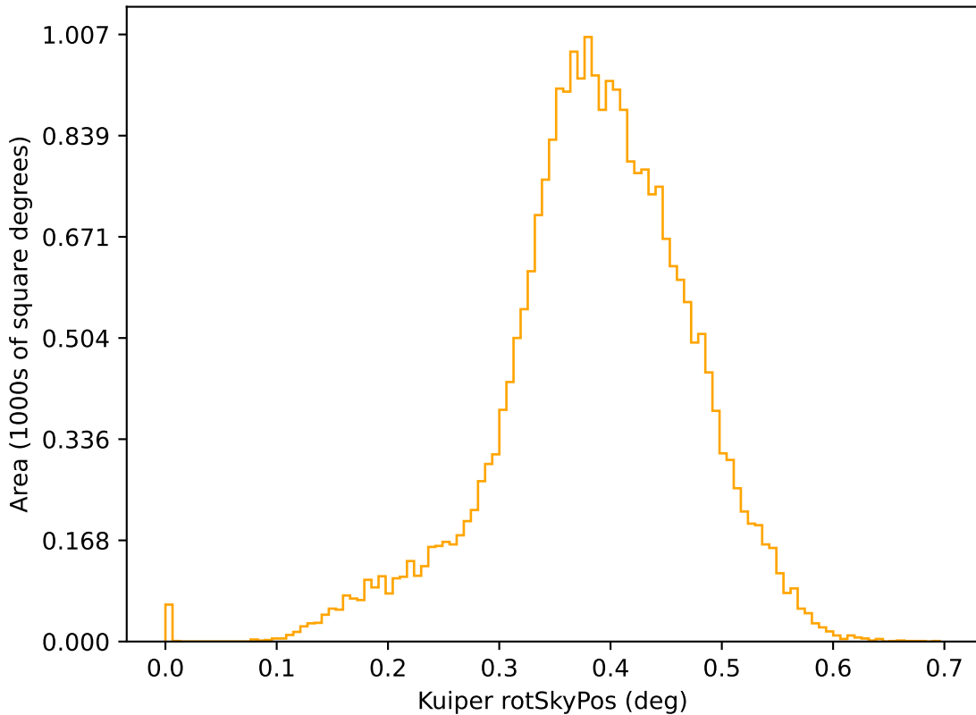
start_date_do-360v3.4_10yrs r: Kuiper rotSkyPos
