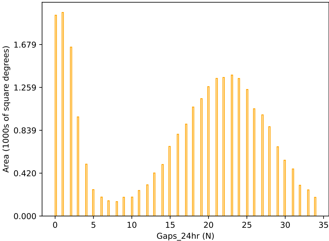
start_date_do-360v3.4_10yrs r band: Gaps_24hr
