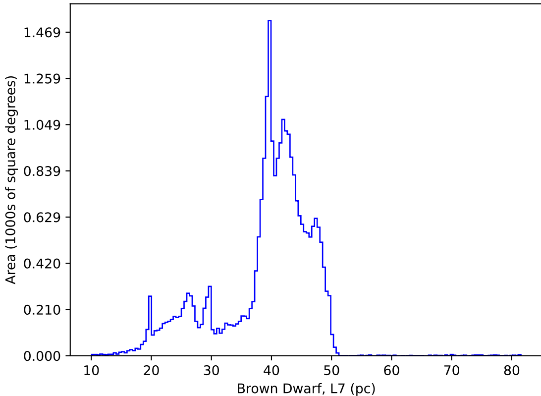
start_date_do-360v3.4_10yrs : Brown Dwarf, L7
