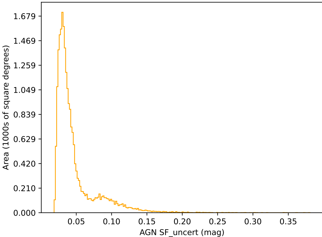
start_date_do-360v3.4_10yrs r band: AGN SF_uncert
