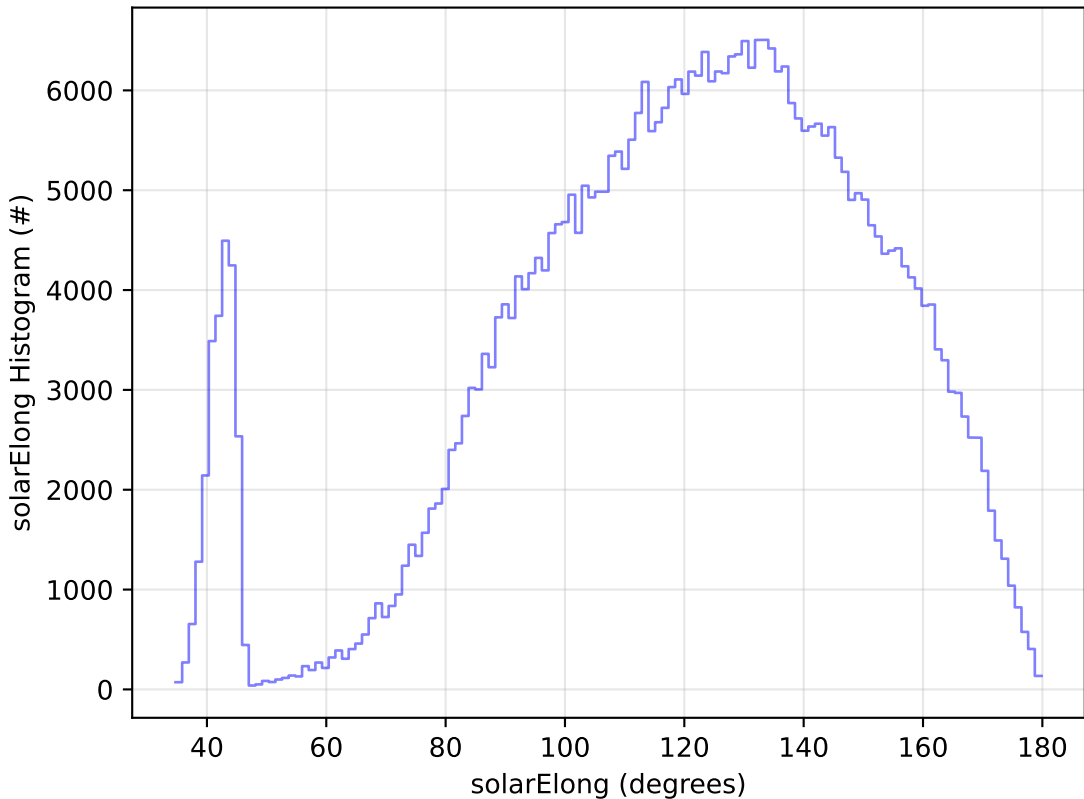
start_date_do-360v3.4_10yrs WFD z band: solarElong Histogram
