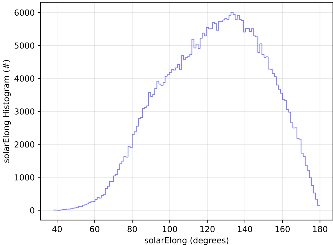
start_date_do-360v3.4_10yrs WFD y band: solarElong Histogram
