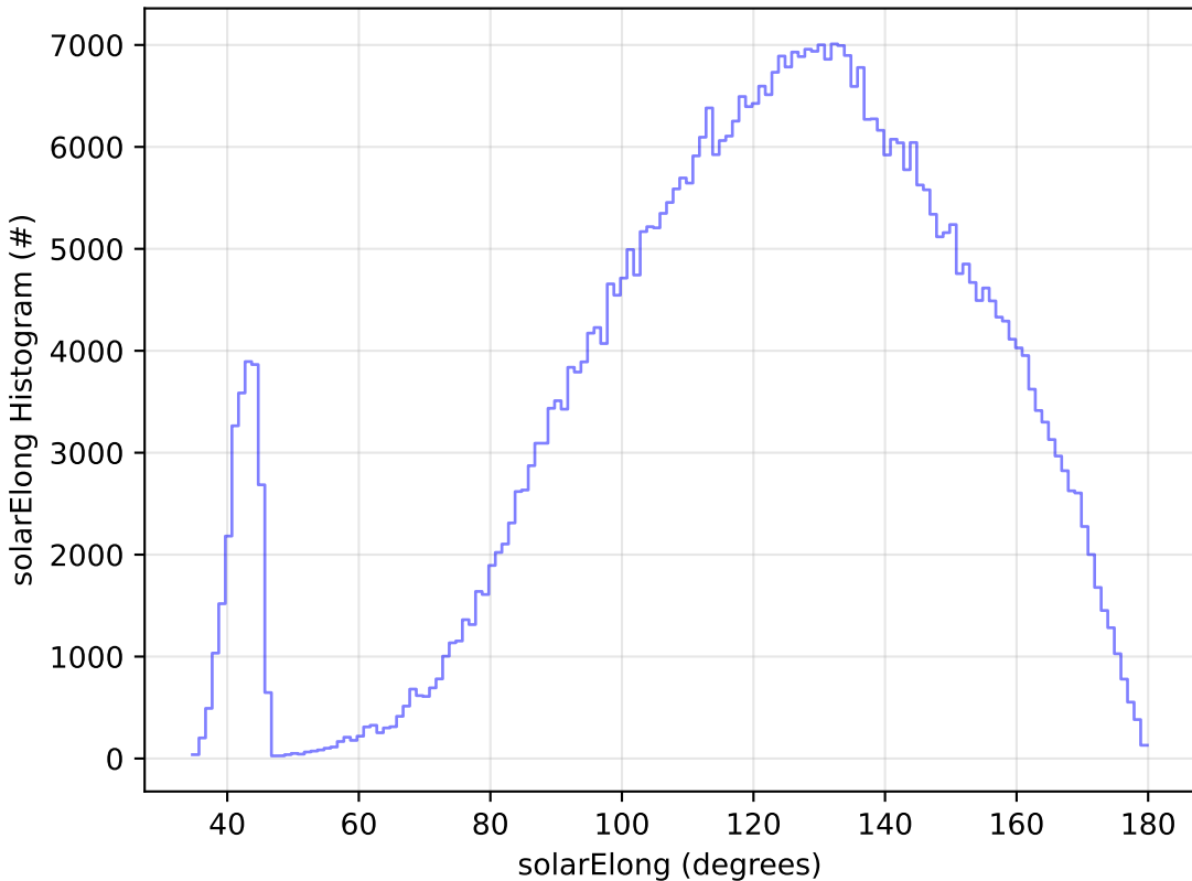
start_date_do-360v3.4_10yrs WFD i band: solarElong Histogram
