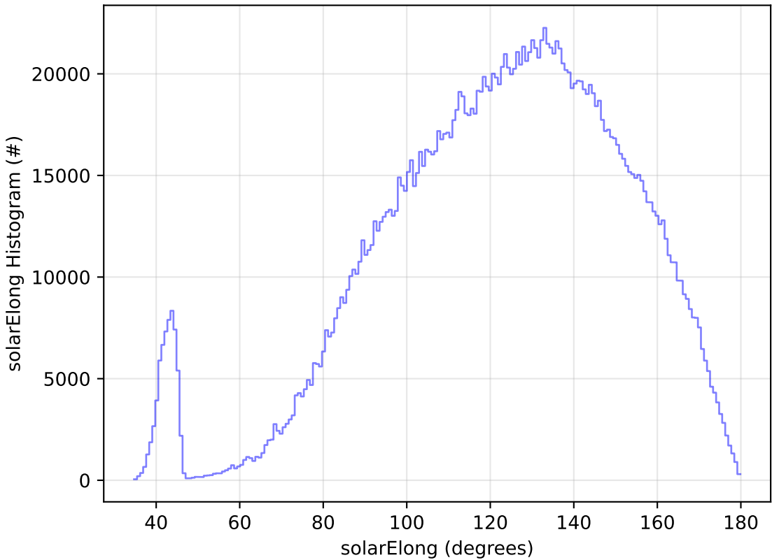
start_date_do-360v3.4_10yrs WFD all bands: solarElong Histogram
