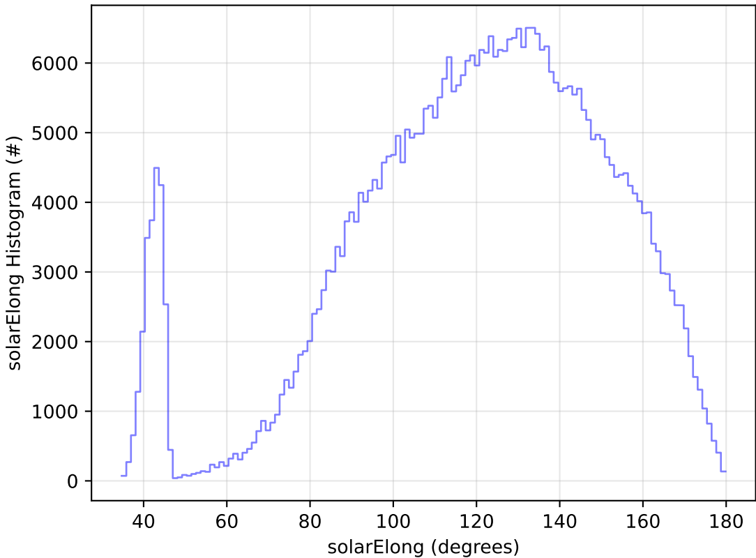
start_date_do-360v3.4_10yrs All sky z band: solarElong Histogram
