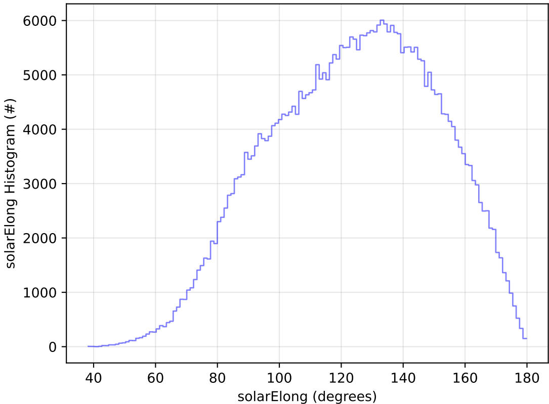
start_date_do-360v3.4_10yrs All sky y band: solarElong Histogram
