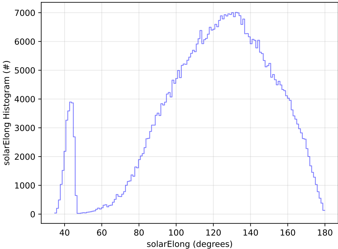
start_date_do-360v3.4_10yrs All sky i band: solarElong Histogram
