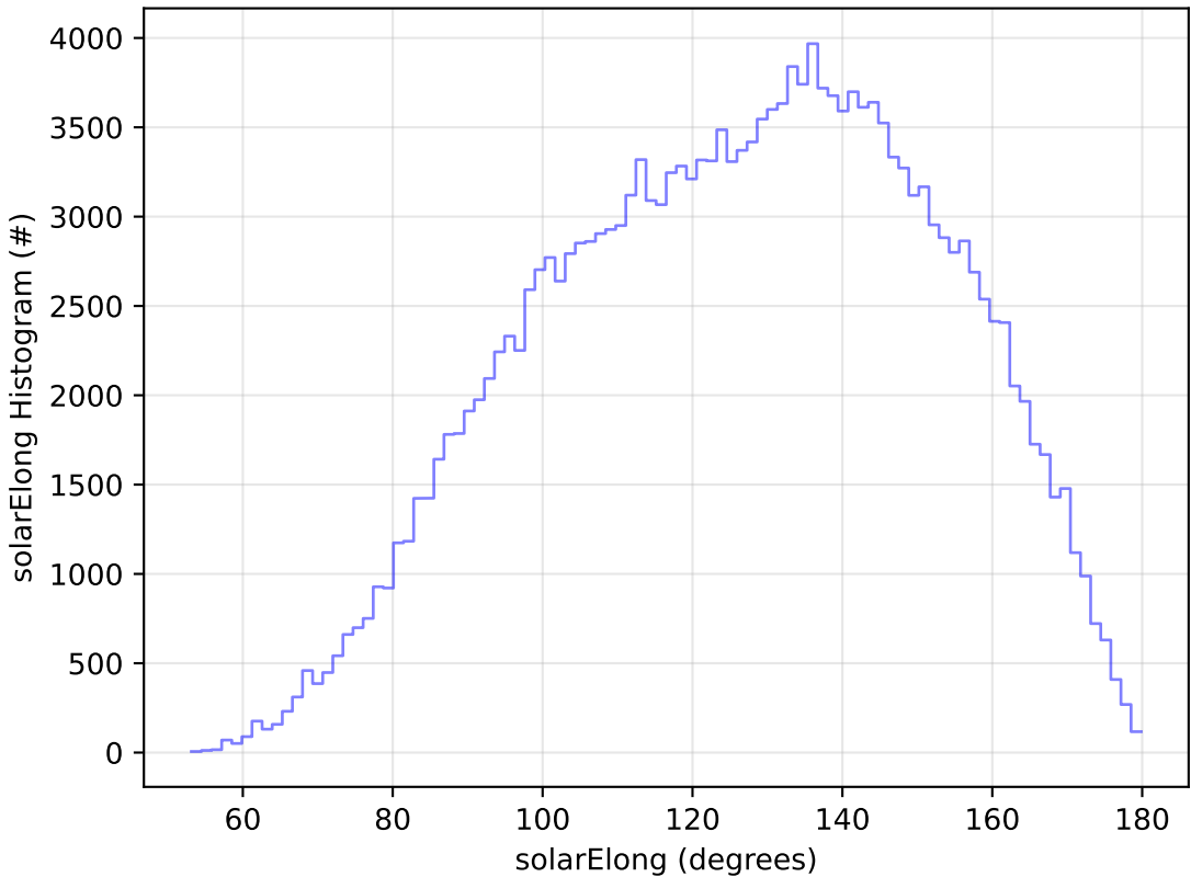
start_date_do-360v3.4_10yrs All sky g band: solarElong Histogram
