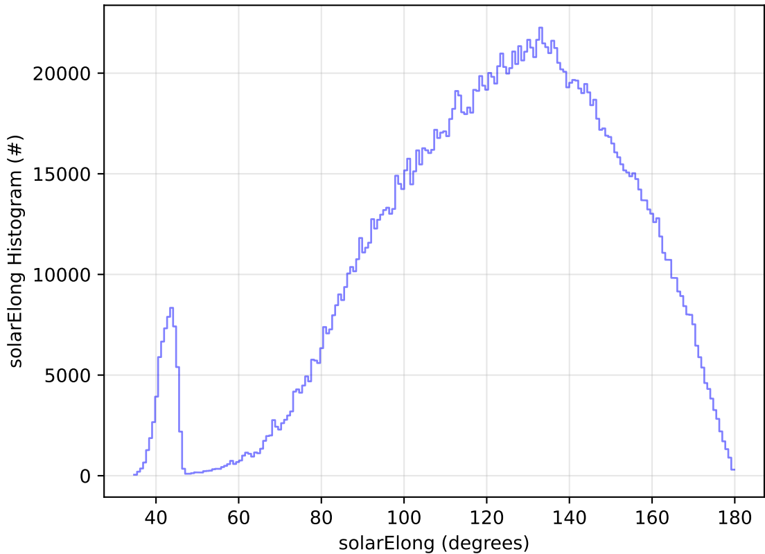
start_date_do-360v3.4_10yrs All sky all bands: solarElong Histogram
