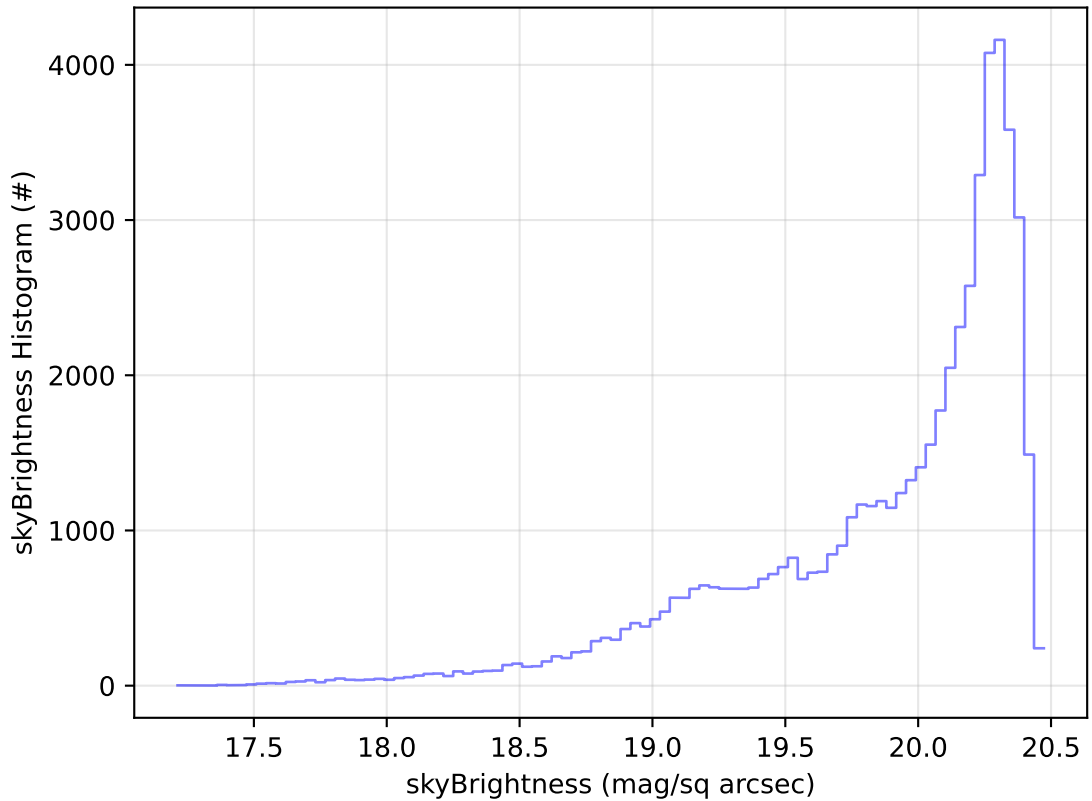
start_date_do-360v3.4_10yrs Yr 1 i band: skyBrightness Histogram
