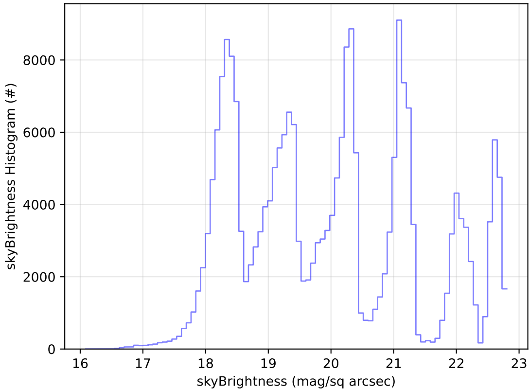
start_date_do-360v3.4_10yrs Yr 1 all bands: skyBrightness Histogram
