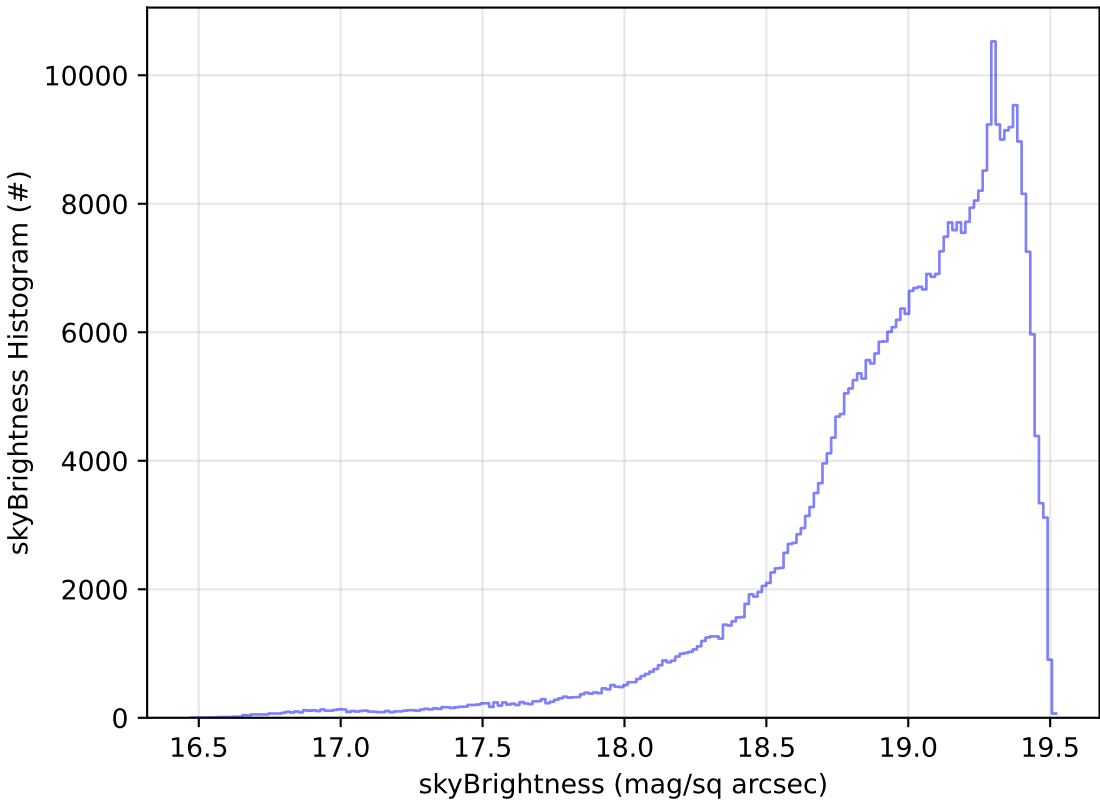
start_date_do-360v3.4_10yrs WFD z band: skyBrightness Histogram
