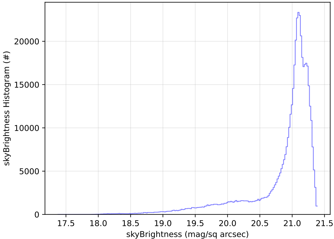
start_date_do-360v3.4_10yrs WFD r band: skyBrightness Histogram
