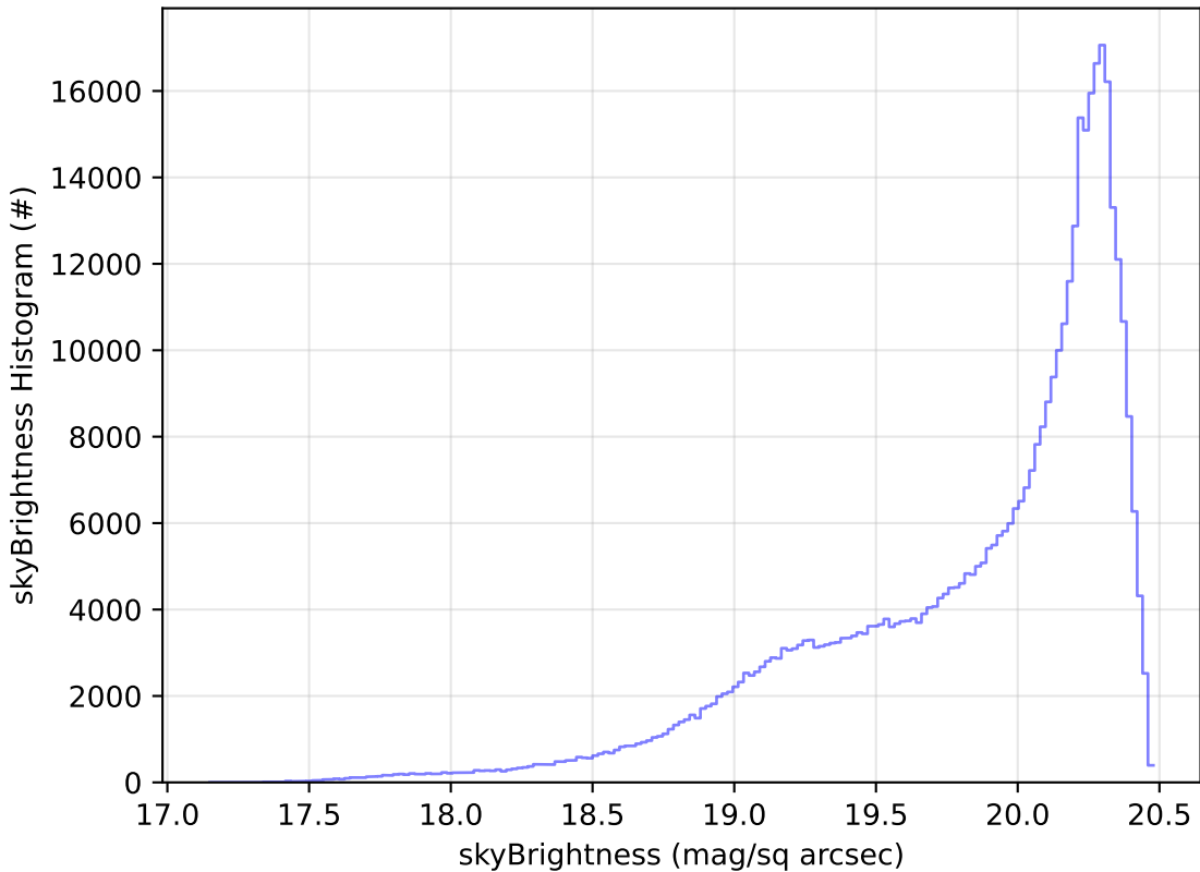
start_date_do-360v3.4_10yrs WFD i band: skyBrightness Histogram
