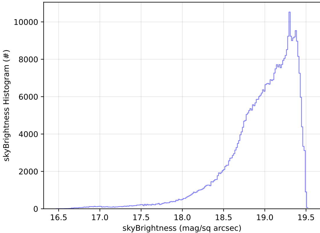
start_date_do-360v3.4_10yrs All sky z band: skyBrightness Histogram
