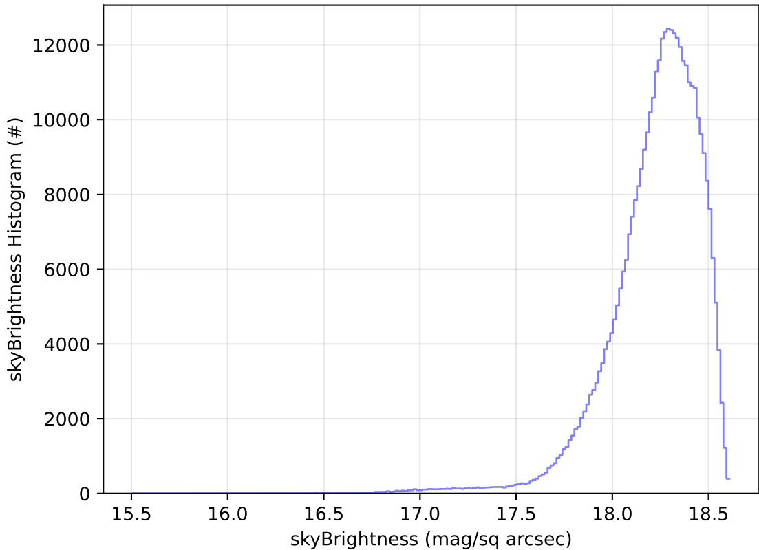
start_date_do-360v3.4_10yrs All sky y band: skyBrightness Histogram
