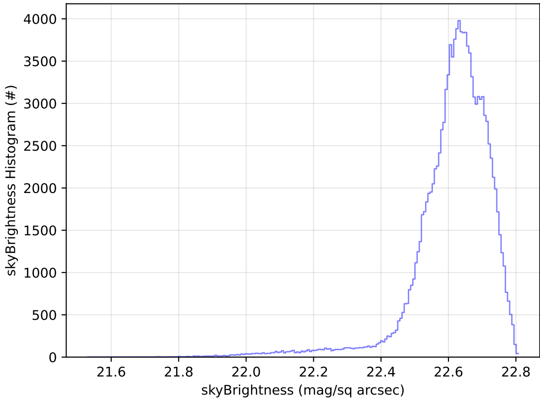
start_date_do-360v3.4_10yrs All sky u band: skyBrightness Histogram
