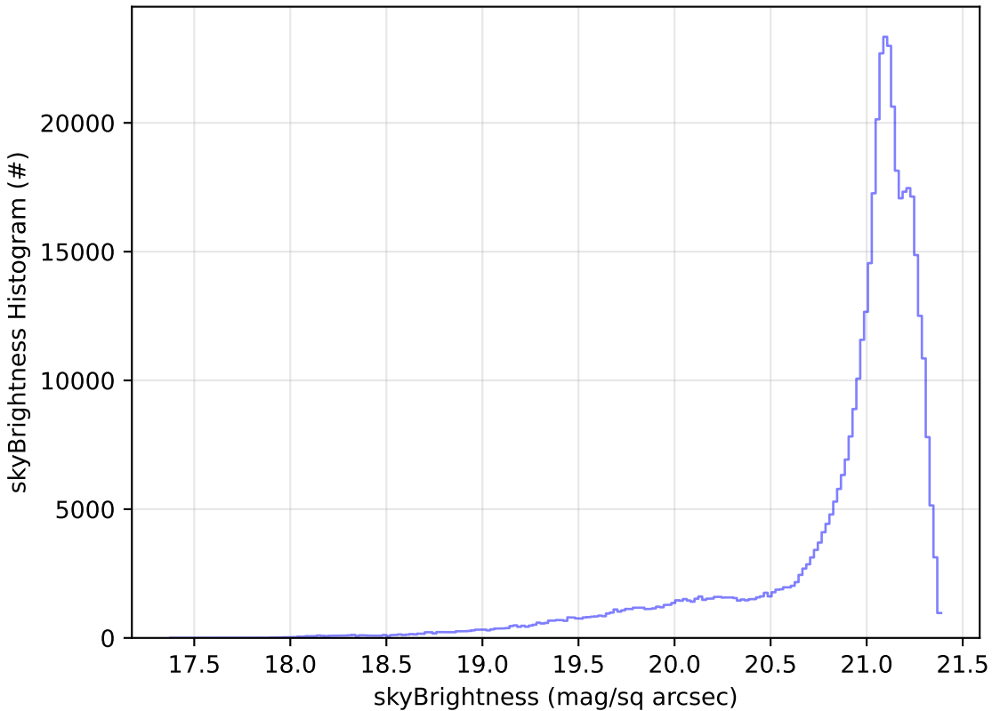
start_date_do-360v3.4_10yrs All sky r band: skyBrightness Histogram
