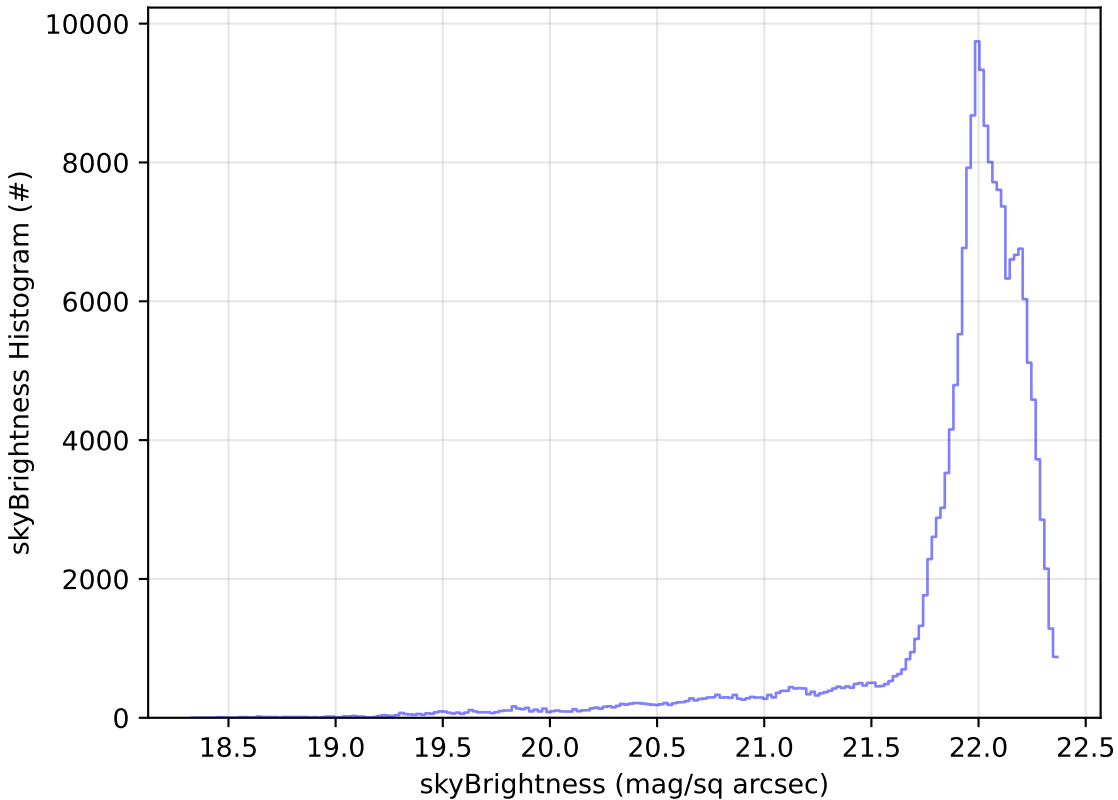
start_date_do-360v3.4_10yrs All sky g band: skyBrightness Histogram
