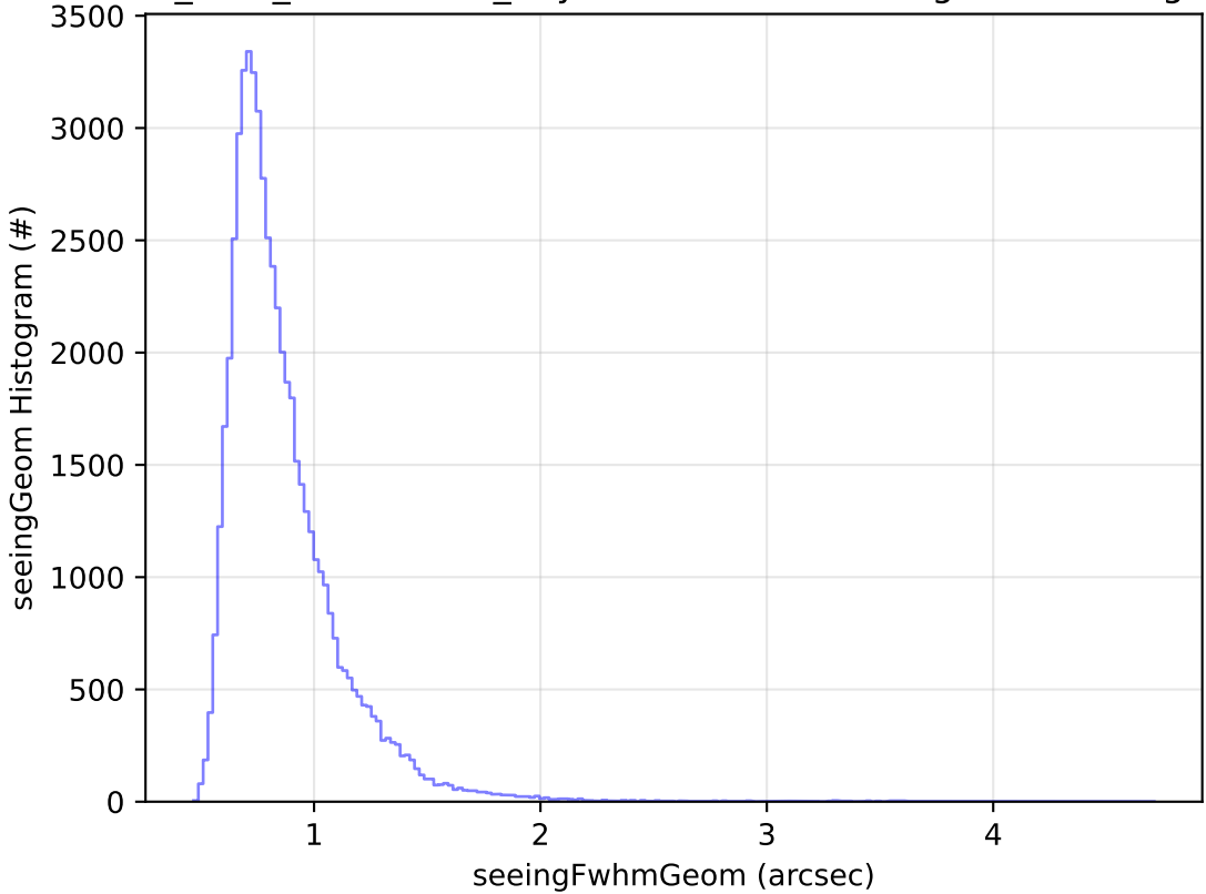
start_date_do-360v3.4_10yrs Yr 1 i band: seeingGeom Histogram
