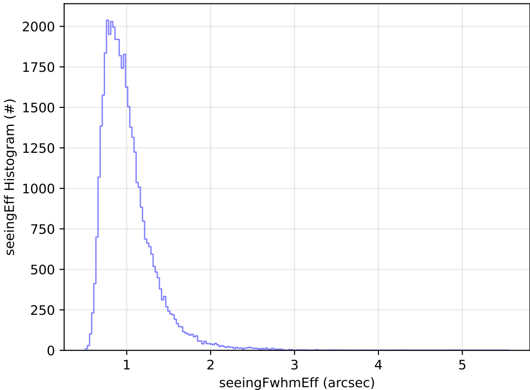
start_date_do-360v3.4_10yrs Yr 1 z band: seeingEff Histogram
