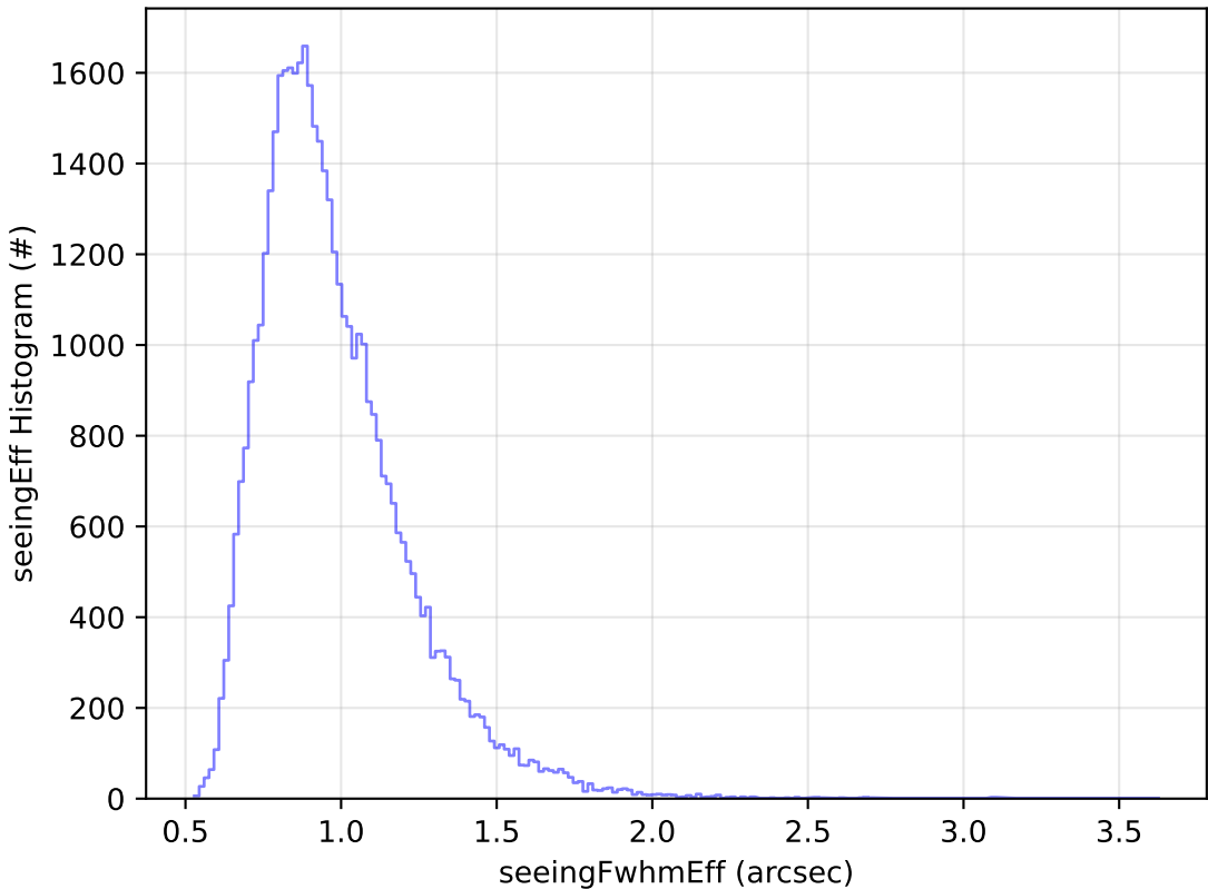
start_date_do-360v3.4_10yrs Yr 1 y band: seeingEff Histogram
