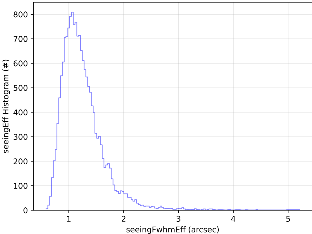
start_date_do-360v3.4_10yrs Yr 1 u band: seeingEff Histogram
