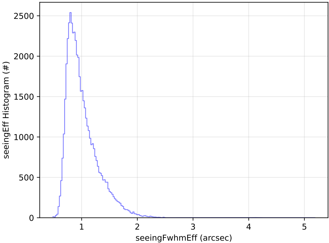
start_date_do-360v3.4_10yrs Yr 1 r band: seeingEff Histogram
