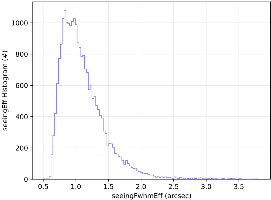
start_date_do-360v3.4_10yrs Yr 1 g band: seeingEff Histogram
