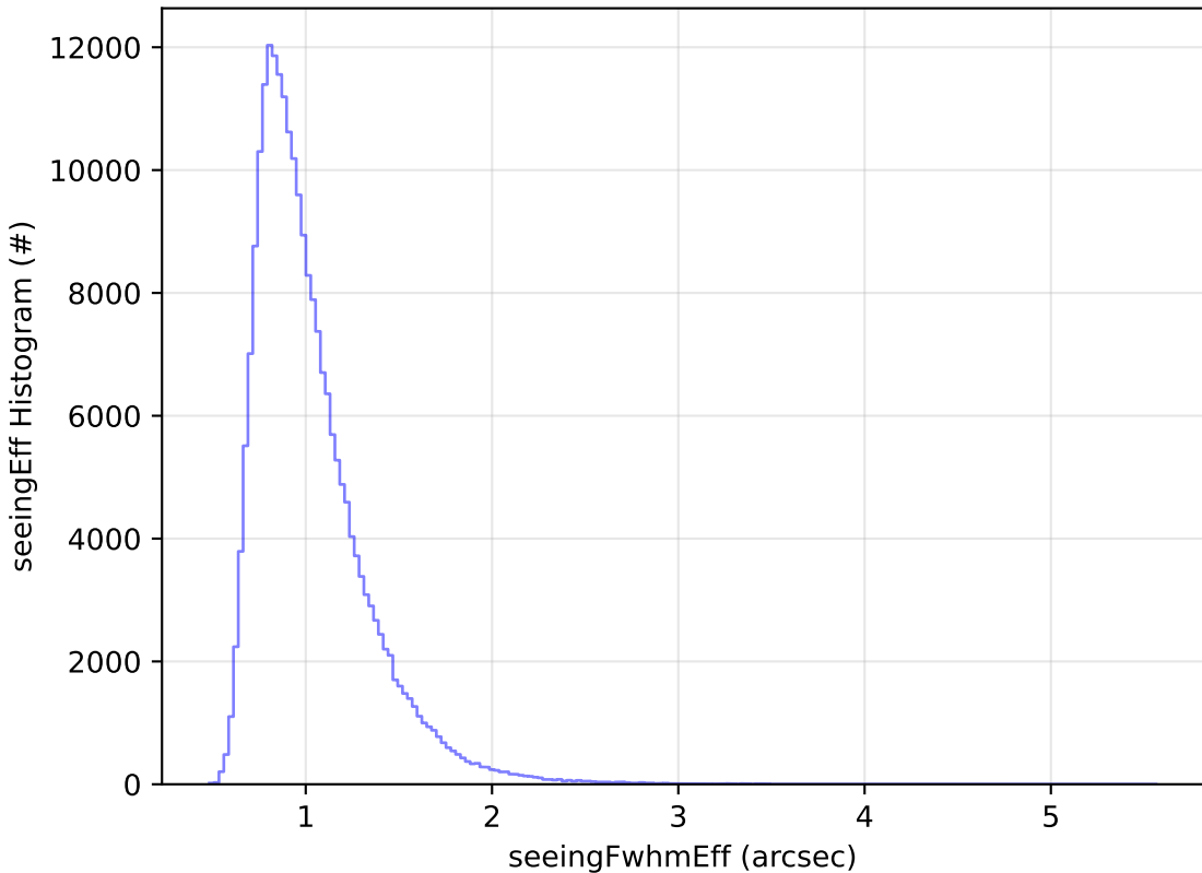
start_date_do-360v3.4_10yrs Yr 1 all bands: seeingEff Histogram
