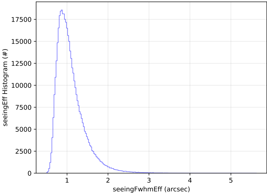
start_date_do-360v3.4_10yrs WFD z band: seeingEff Histogram
