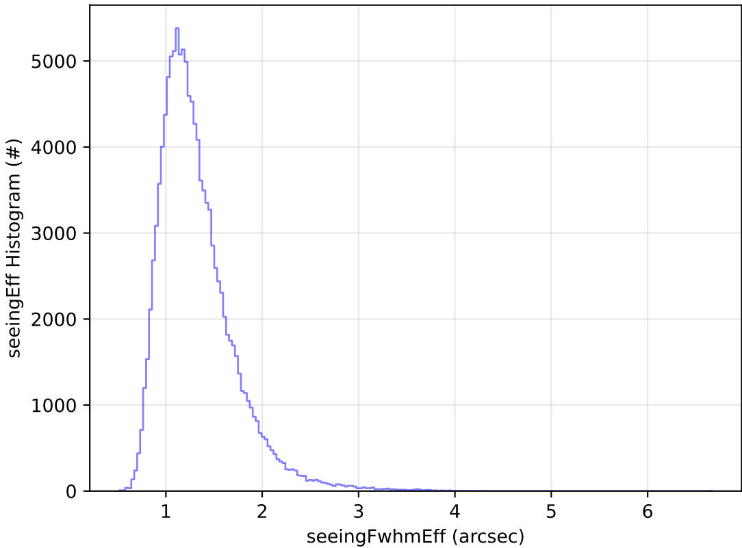
start_date_do-360v3.4_10yrs WFD u band: seeingEff Histogram
